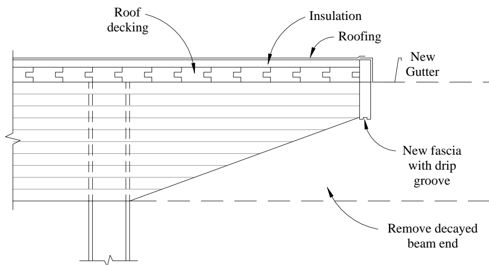
Figure 1. Removal of decayed beam end.
