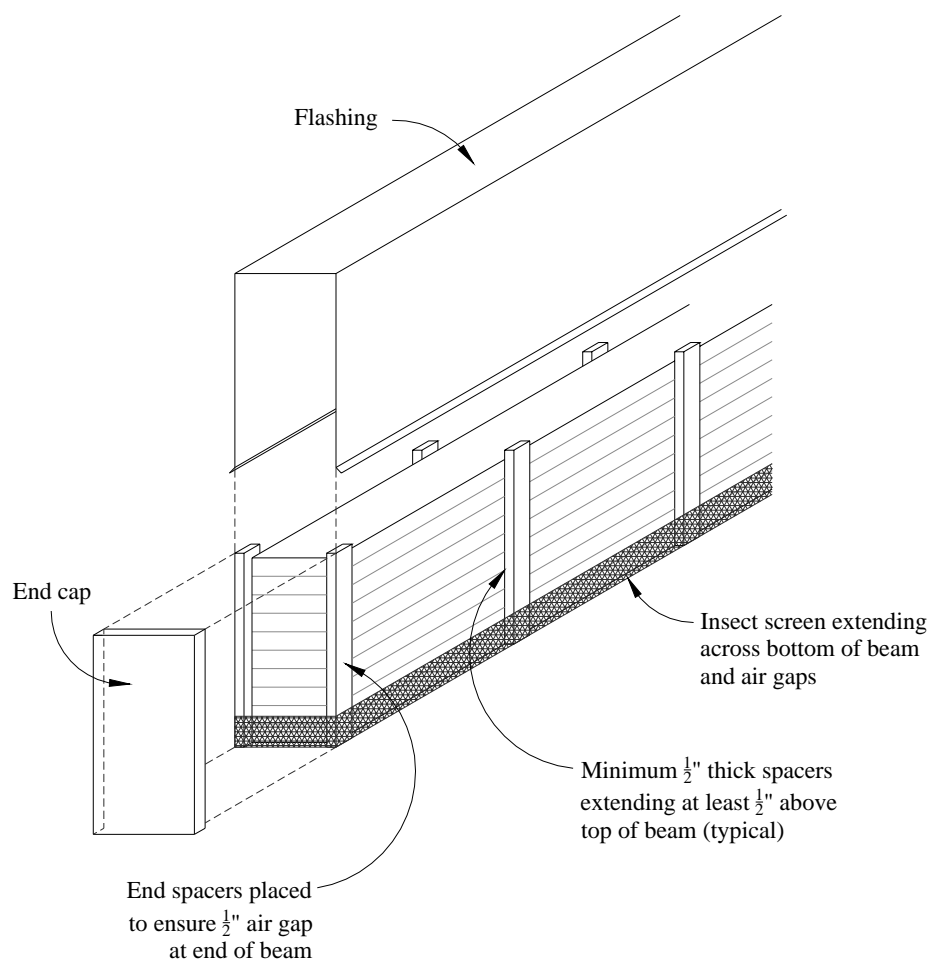
Figure 2. Metal cover protection for glued laminated beam.
